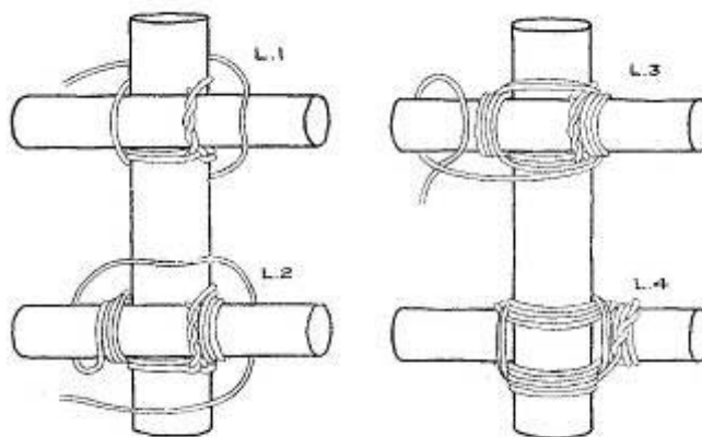
SQUARE LASHING
